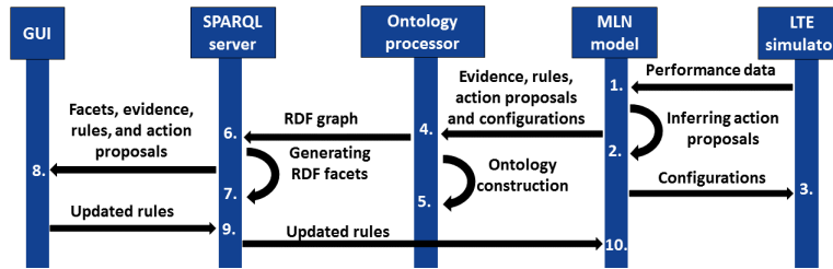
Fig. 1. Data sequence diagram for managing a mobile network (simulator)
